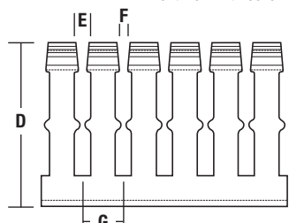
Figure 2: Side View without Cover
