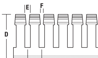
Figure 1: Side View without Cover
