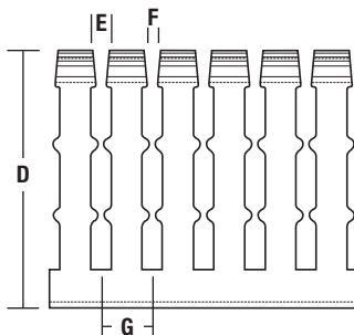
Figure 3: Side View without Cover
